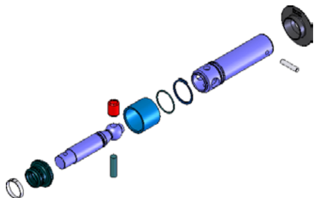
Shaft/Rod Assembly
