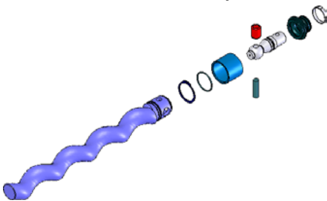
Rotor/Rod Assembly
